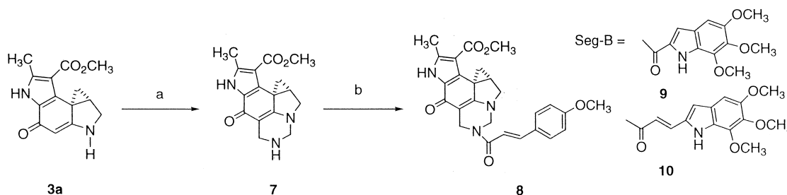
Scheme 2. (a) HMT, TFA, rt, (57%); (b) 4-methoxycinnamic acid (70%) or 5,6,7-trimethoxy-2-indolecarboxylic acid (76%) or 3-(5,6,7-trimethoxy-2-indole)acrylic acid (43%), EDCI, \text{CH}_2\text{Cl}_2 , rt.
